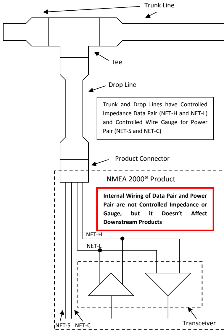
NMEA 2000® Approved Wiring
