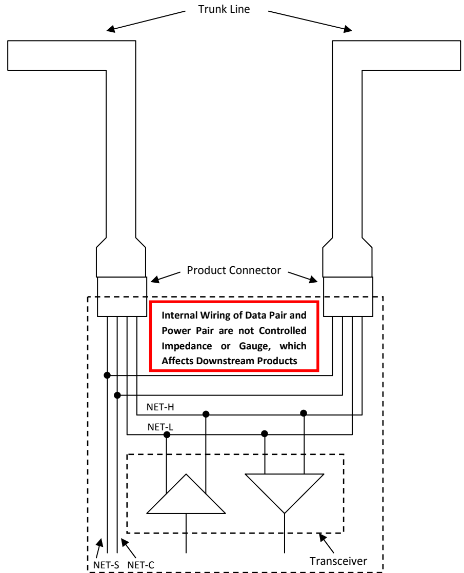
Daisy Chaining (Not NMEA 2000® Approved)
